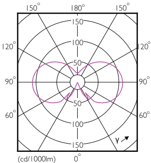
Light Distribution Diagram - CLA LEDLuster ND 2.2-25W P45 E27 FR
