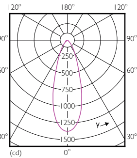
Light Distribution Diagram - MAS LED spot VLE D 7-80W GU10 865 36D
