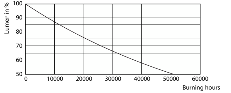
Lumen Maintenance Diagram - MAS LED spot VLE D 650lm GU10 830 120D
