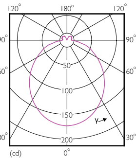
Light Distribution Diagram - MAS LED spot VLE D 680lm GU10 840 120D
