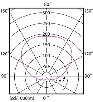
Light Distribution Diagram - CorePro LEDbulb D 13.5-100W A67 E27 827
