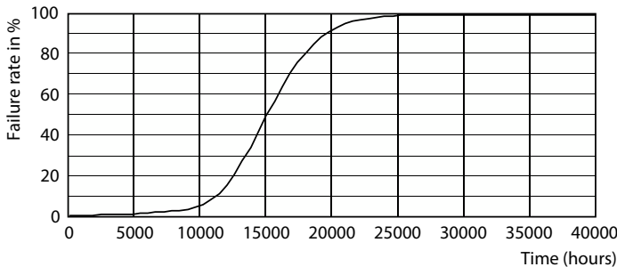
Life Expectancy Diagram - ESS LEDBulb 12W E27 3000K 1PF/6 MX
