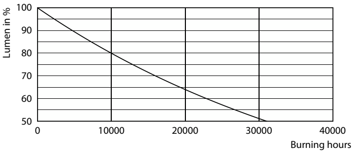
Lumen Maintenance Diagram - ESS LEDBulb 12W E27 3000K 1PF/6 MX
