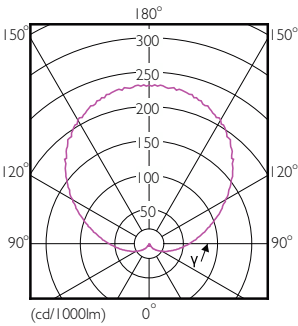
Light Distribution Diagram - ESS LEDBulb 12W E27 3000K 1PF/6 MX
