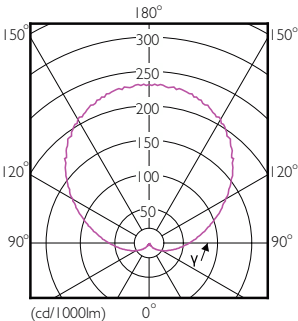
Light Distribution Diagram - ESS LEDBulb 12W E27 6500K 1PF/6 MX
