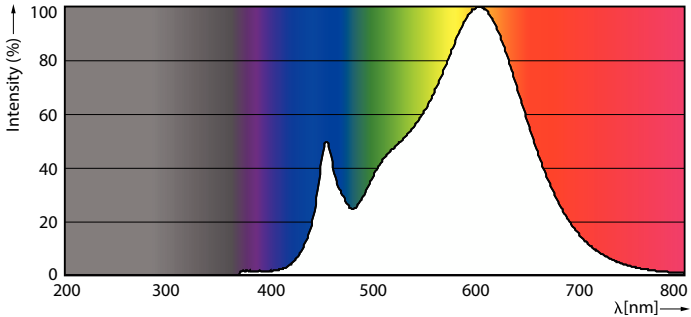
Spectral Power Distribution Colour - Master LED PAR30L 20W 15D 830
