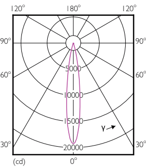
Light Distribution Diagram - Master LED PAR30L 20W 15D 840
