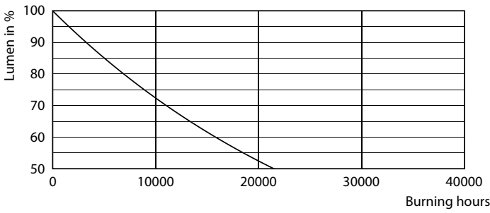
Lumen Maintenance Diagram - LEDBulb 14.5W E27 3000K 230V A67 APR
