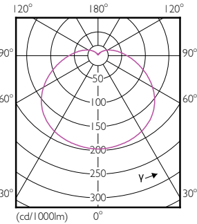
Light Distribution Diagram - LEDBulb 14.5W E27 3000K 230V A67 APR
