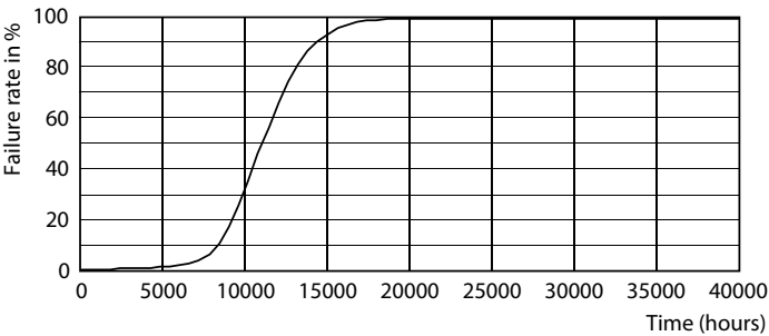
Life Expectancy Diagram - LEDBulb 14.5W E27 3000K 230V A67 APR
