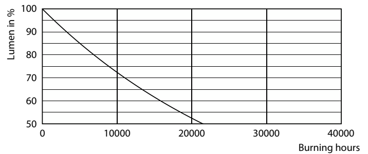
Lumen Maintenance Diagram - LEDBulb 14.5W E27 6500K 230V A67 APR
