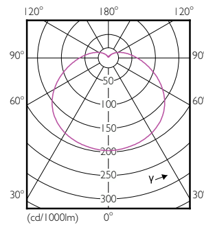
Light Distribution Diagram - LEDBulb 14.5W E27 6500K 230V A67 APR
