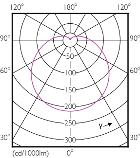
Light Distribution Diagram - LEDBulb 19W E27 6500K 230V A80 APR
