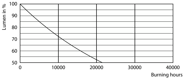
Lumen Maintenance Diagram - LEDBulb 19W E27 6500K 230V A80 APR
