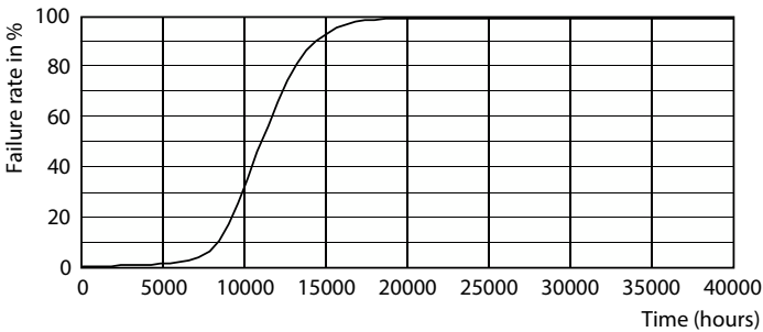
Life Expectancy Diagram - LEDBulb 19W E27 6500K 230V A80 APR
