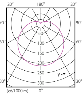
Light Distribution Diagram - LEDBulb 19W E27 6500K 230V A80 APR
