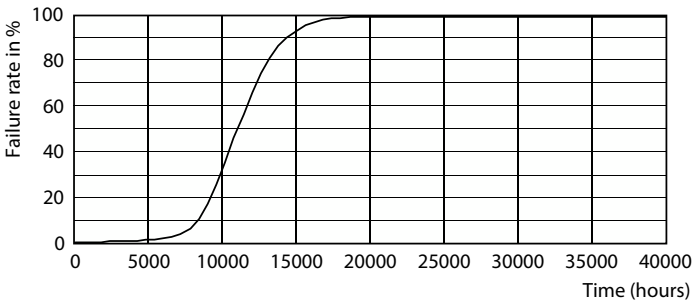
Life Expectancy Diagram - LEDBulb 19W E27 6500K 220-240V A80 AR
