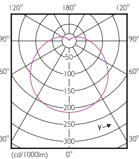
Light Distribution Diagram - LEDBulb 19W E27 6500K 220-240V A80 AR
