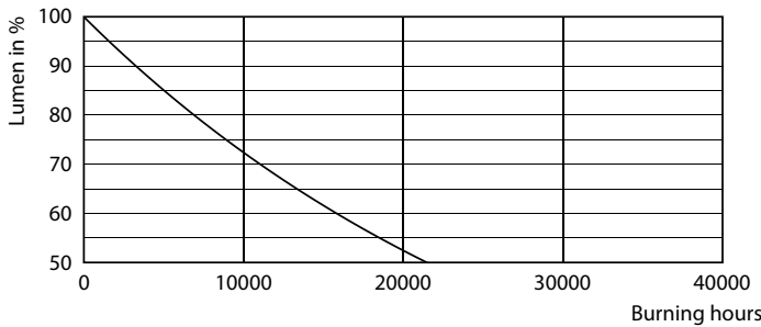
Lumen Maintenance Diagram - LEDBulb 19W E27 6500K 220-240V A80 AR
