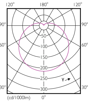
Light Distribution Diagram - LEDBulb 40W E40 6500K 230V A130 APR
