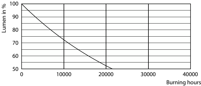
Lumen Maintenance Diagram - LEDBulb 40W E40 6500K 230V A130 APR
