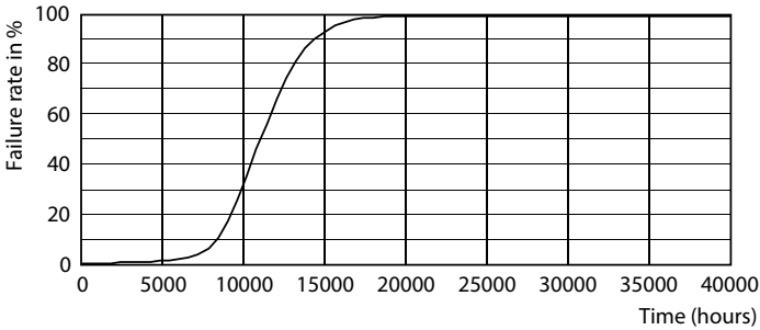
Life Expectancy Diagram - LEDBulb 40W E40 6500K 230V A130 APR
