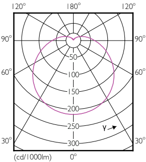
Light Distribution Diagram - LEDBulb 40W E40 6500K 230V A130 APR
