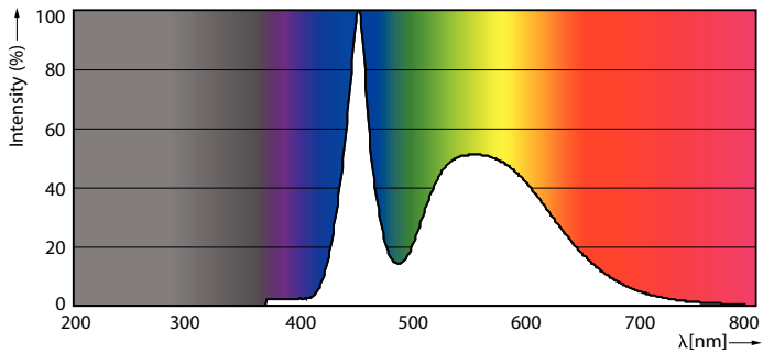
Spectral Power Distribution Colour - LEDBulb 40W E40 6500K 230V A130 APR
