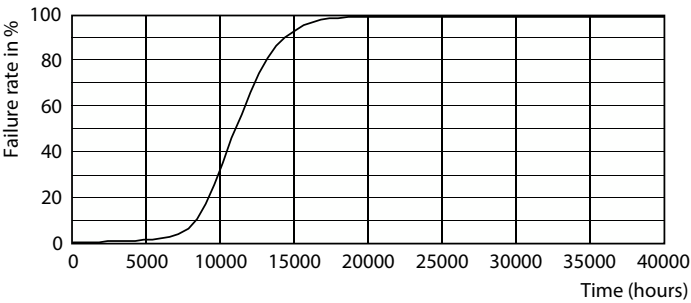
Life Expectancy Diagram - LEDBulb 40W E40 6500K 230V A130 APR
