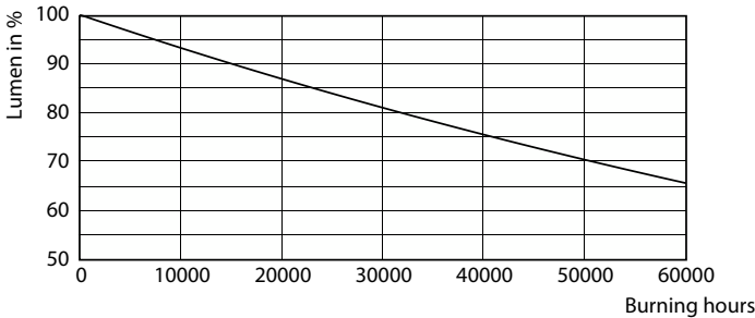
Lumen Maintenance Diagram - TForce LED HPI ND 200-145W E40 840 60D
