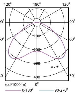
Light Distribution Diagram - TForce LED HPI ND 200-145W E40 840 120D
