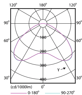
Light Distribution Diagram - TForce LED HPI ND 200-145W E40 840 120D
