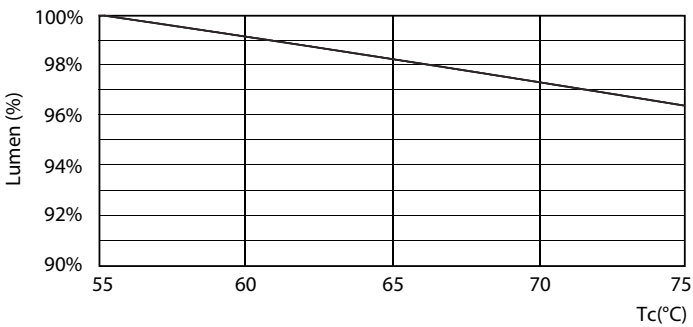
Lumen Maintenance Diagram - 17T8 PRO LED/48-3000 BB G 1PK 10/1
