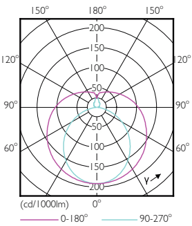
Light Distribution Diagram - 17T8 PRO LED/48-3000 BB G 1PK 10/1
