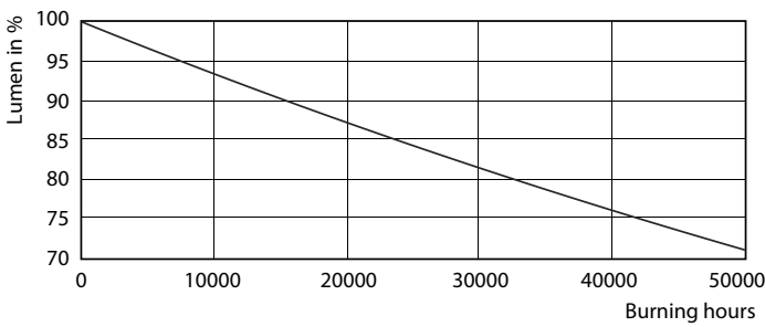
Lumen Maintenance Diagram - 17T8 PRO LED/48-3000 BB G 1PK 10/1
