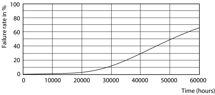
Life Expectancy Diagram - 17T8 PRO LED/48-3000 BB G 1PK 10/1
