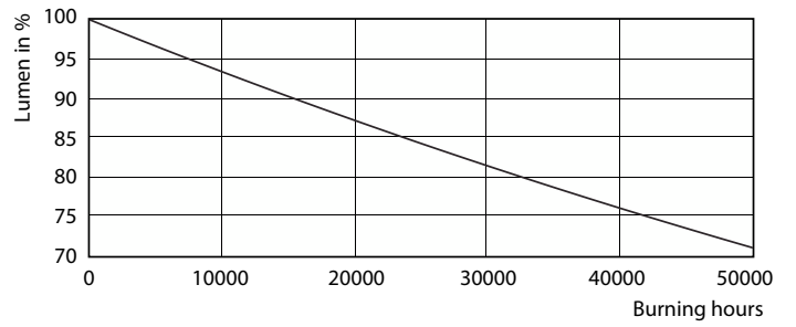
Lumen Maintenance Diagram - 16.5T8PRO/48-830/BB20/G 10/1 FB
