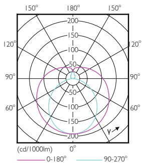
Light Distribution Diagram - 16.5T8PRO/48-830/BB20/G 10/1 FB
