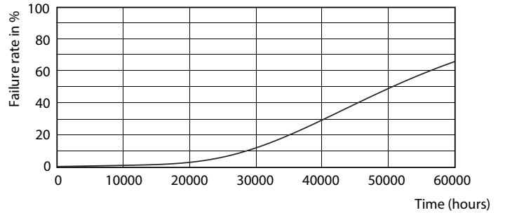
Life Expectancy Diagram - 16.5T8PRO/48-830/BB20/G 10/1 FB
