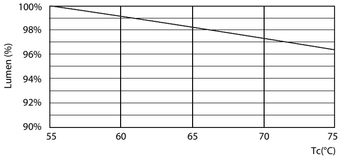
Lumen Maintenance Diagram - 16.5T8PRO/48-830/BB20/G 10/1 FB
