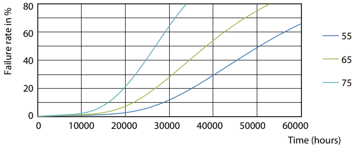
Life Expectancy Diagram - 16.5T8PRO/48-830/BB20/G 10/1 FB
