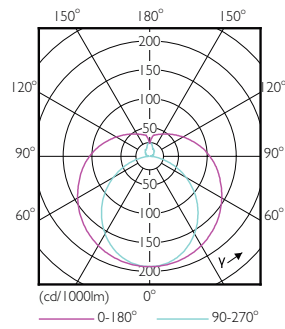
Light Distribution Diagram - 16.5T8PRO/48-835/BB20/G 10/1 FB
