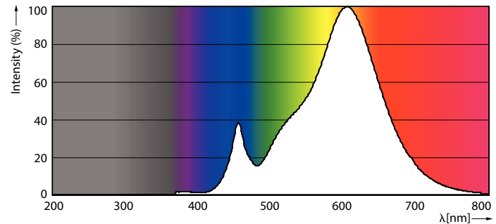
Spectral Power Distribution Colour - Master LED PAR30L 40W 15D 827
