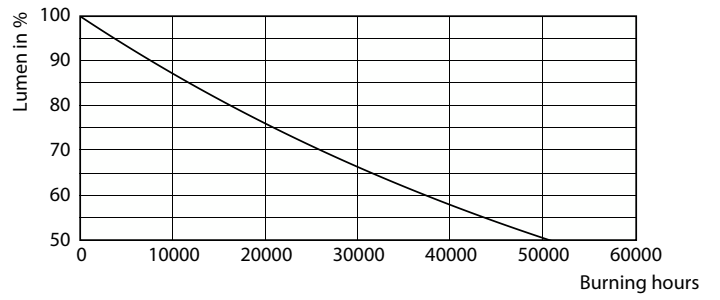
Lumen Maintenance Diagram - Master LED PAR30L 40W 15D 827
