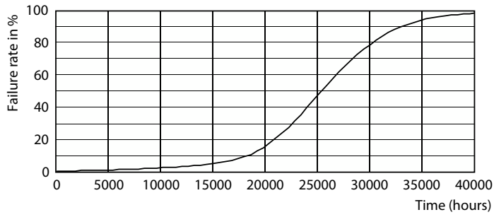
Life Expectancy Diagram - Master LED PAR30L 40W 15D 827
