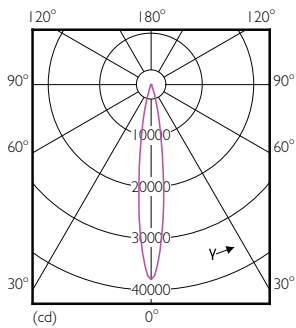
Light Distribution Diagram - Master LED PAR30L 40W 15D 827
