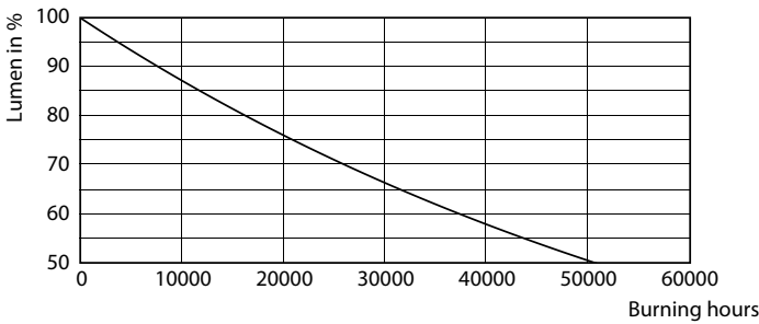
Lumen Maintenance Diagram - Master LED PAR30L 40W 15D 830 CN
