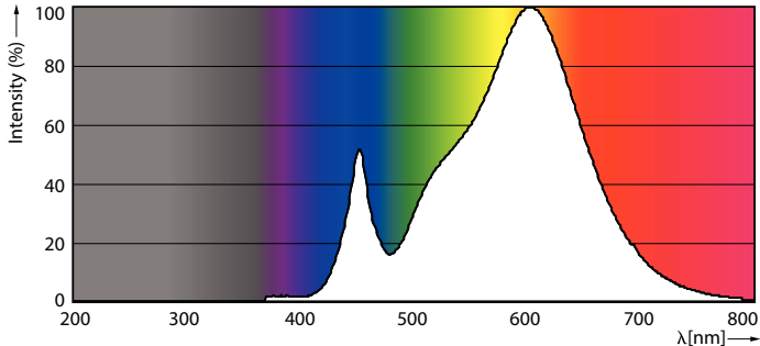
Spectral Power Distribution Colour - Master LED PAR30L 40W 15D 830 CN
