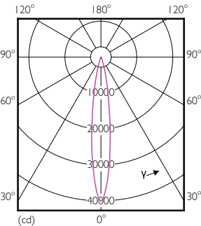
Light Distribution Diagram - Master LED PAR30L 40W 15D 830 CN
