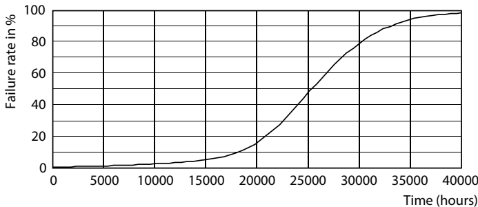
Life Expectancy Diagram - Master LED PAR30L 40W 15D 857
