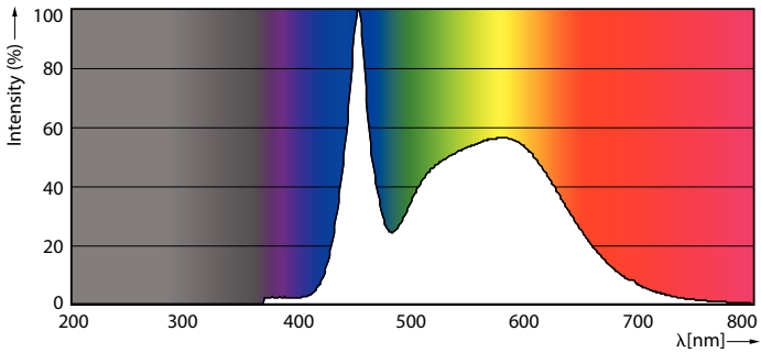
Spectral Power Distribution Colour - Master LED PAR30L 40W 15D 857
