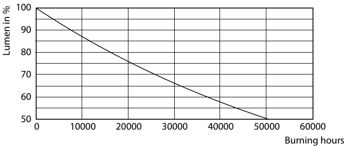
Lumen Maintenance Diagram - Master LED PAR30L 40W 15D 857
