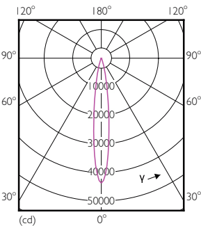
Light Distribution Diagram - Master LED PAR30L 40W 15D 857
