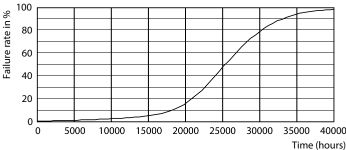
Life Expectancy Diagram - Master LED PAR30L 40W 15D 860 CN
