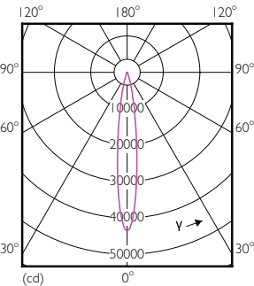
Light Distribution Diagram - Master LED PAR30L 40W 15D 860 CN
