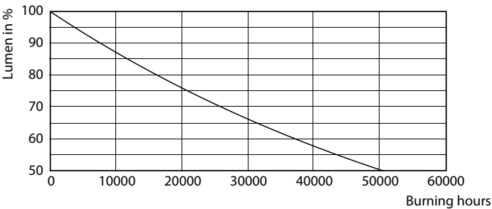
Lumen Maintenance Diagram - Master LED PAR30L 40W 15D 860 CN
