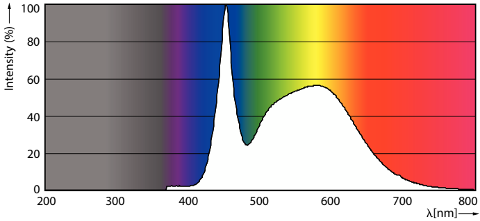
Spectral Power Distribution Colour - Master LED PAR30L 40W 15D 860 CN
