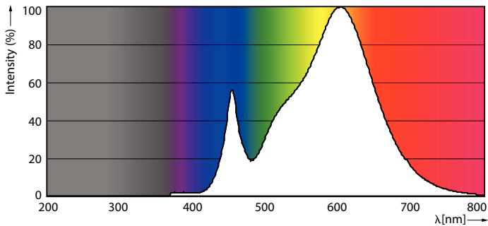
Spectral Power Distribution Colour - Master LED PAR30L 40W 30D 830
