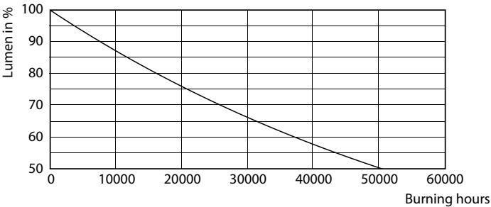
Lumen Maintenance Diagram - Master LED PAR30L 40W 30D 857
