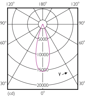
Light Distribution Diagram - Master LED PAR30L 40W 30D 857
