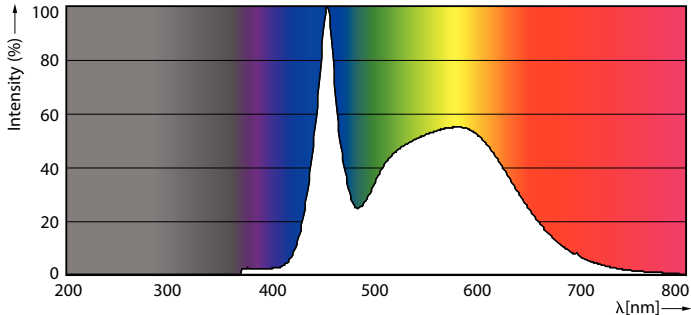
Spectral Power Distribution Colour - Master LED PAR30L 40W 30D 857
