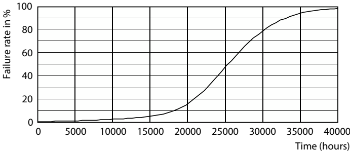
Life Expectancy Diagram - Master LED PAR30L 40W 30D 857
