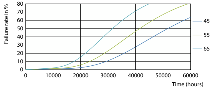
Life Expectancy Diagram - MAS LEDtube 1200mm 14W 840 T8 THD
