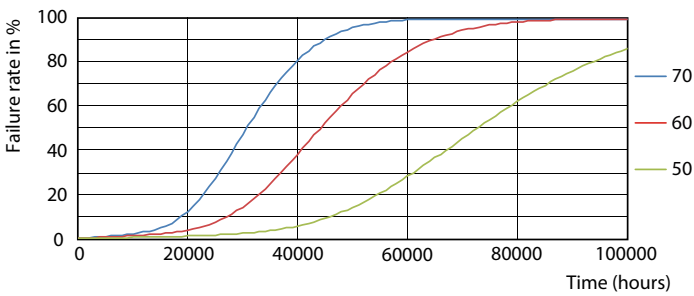
LEDtube G13 ND FailureRate
