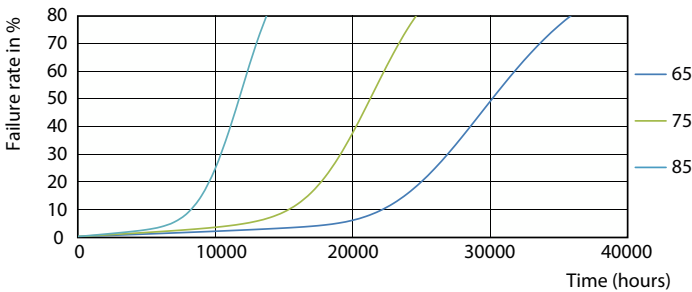
Life Expectancy Diagram - CorePro LEDtube 1200mm 16W865 G5 I APR
