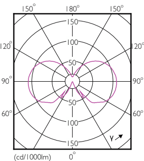
Light Distribution Diagram – LEDClassic SSW 60W A60 B22 WW CL ND 1SRT
