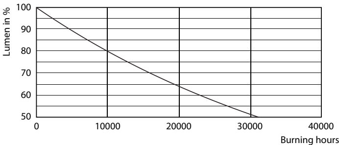
Lumen Maintenance Diagram - LEDClassic SSW 60W A60 B22 WW CL ND 1SRT
