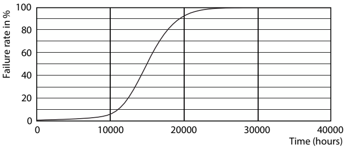
Life Expectancy Diagram - LEDClassic SSW 60W A60 B22 WW CL ND 1SRT
