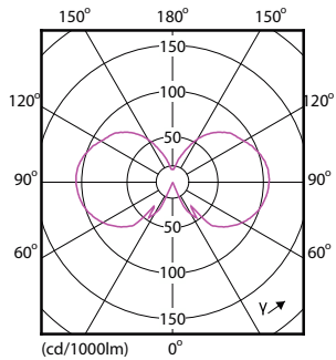
Light Distribution Diagram - CLA LEDBulb ND 8-75W E27 WW A60 CL
