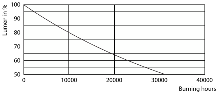
Lumen Maintenance Diagram - CLA LEDBulb ND 11-100W E27 WW A67 CL
