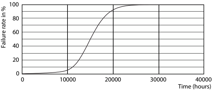
Life Expectancy Diagram - CLA LEDBulb ND 11-100W E27 WW A67 CL
