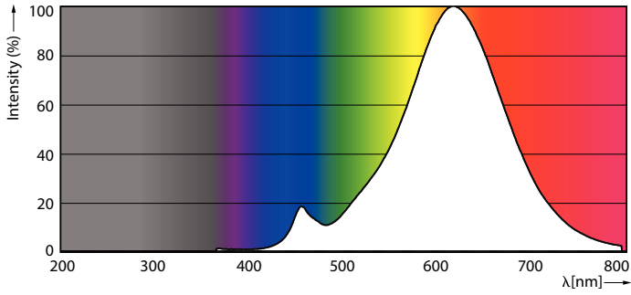
Spectral Power Distribution Colour - LEDClassic 7-70W A60 E27 WW CL ND APR
