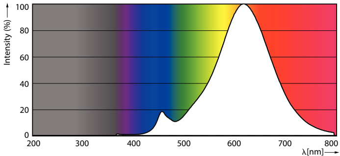
Spectral Power Distribution Colour - CLA LEDBulb ND 7-60W B22 WW A60 CL
