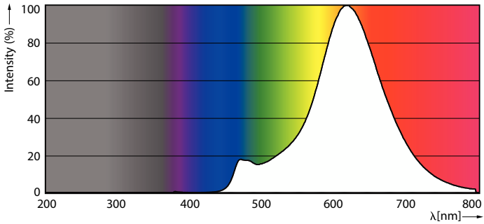
Spectral Power Distribution Colour - CLA LEDBulb SP ND 5-25W E27 GOLD ST64 CL
