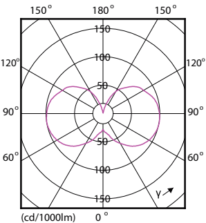
Light Distribution Diagram - CLA LEDBulb SP ND 5-25W E27 GOLD ST64 CL
