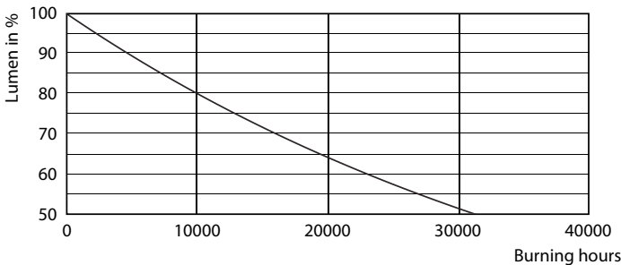
Lumen Maintenance Diagram - LED classic SP 25W G93 E27 GOLD ND 1PF/4
