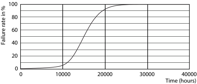
Life Expectancy Diagram - LED classic SP 25W G93 E27 GOLD ND 1PF/4
