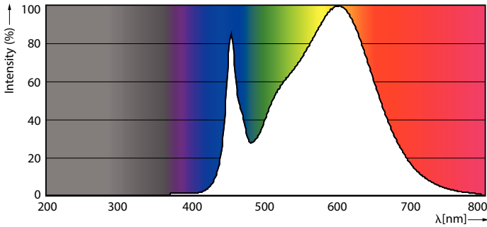
Spectral Power Distribution Colour - 15T8/24-835/IF20-6U/MAScon IA 10/1
