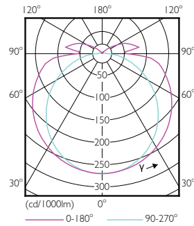
Light Distribution Diagram - 15T8/24-835/IF20-6U/MAScon IA 10/1
