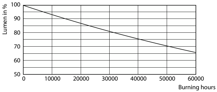
Lumen Maintenance Diagram - 15T8 LED/24-4000 IF 6U EasySmart 1PK
