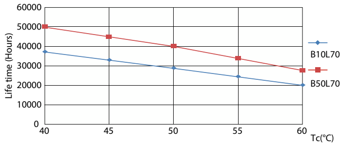
Life Expectancy Diagram - 15T8 LED/24-4000 IF 6U EasySmart 1PK
