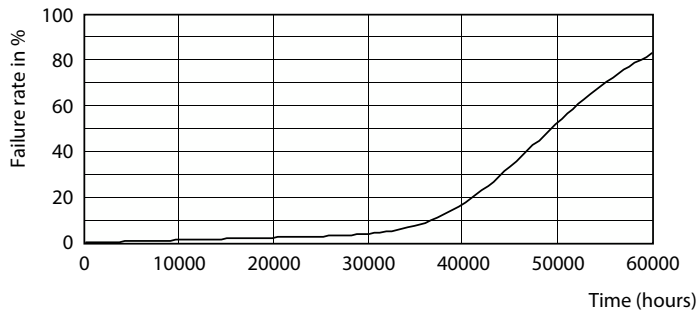
Life Expectancy Diagram - 15T8 LED/24-4000 IF 6U EasySmart 1PK
