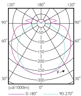
Light Distribution Diagram - 15T8 LED/24-4000 IF 6U EasySmart 1PK
