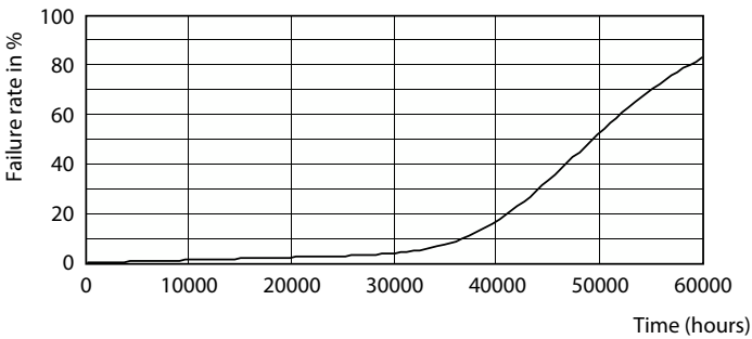
Life Expectancy Diagram - 8T8 LED/24-5000 IF EasySmart 1PK
