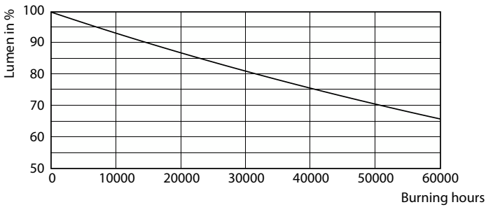
Lumen Maintenance Diagram - 8T8 LED/24-5000 IF EasySmart 1PK
