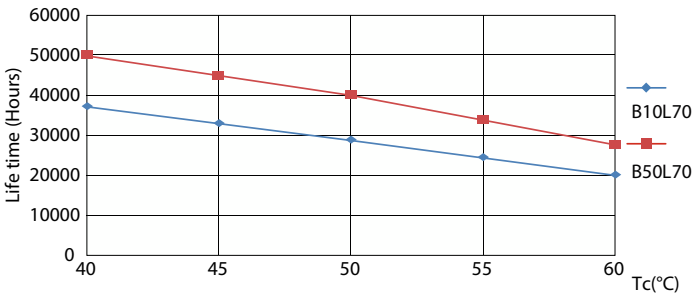
Life Expectancy Diagram - 8T8 LED/24-5000 IF EasySmart 1PK
