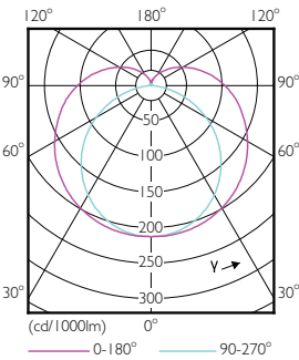
Light Distribution Diagram - 8T8 LED/24-5000 IF EasySmart 1PK
