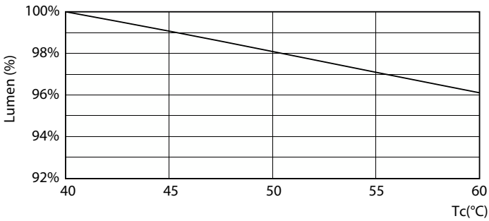
Lumen Maintenance Diagram - 8T8 LED/24-5000 IF EasySmart 1PK
