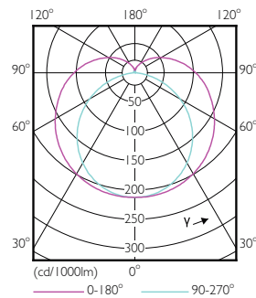
Light Distribution Diagram - 8T8/24-850/IF12/MAScon IA 10/1
