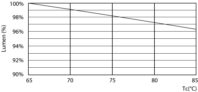
Lumen Maintenance Diagram - MAS LEDtube 1200mm 17W 865 T8 I W G
