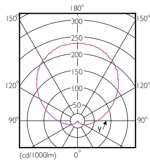
Light Distribution Diagram - Ess LEDBulb 3.5-25W E27 3000K A19 1PK MX
