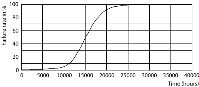
Life Expectancy Diagram - Ess LEDBulb 8-60W E27 3000K A19 1PK MX
