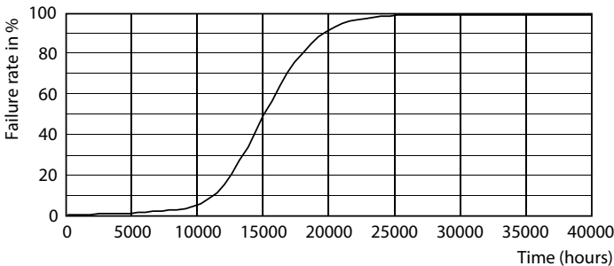
Life Expectancy Diagram - Ess LEDBulb 8-60W E27 6500K A19 1PK MX
