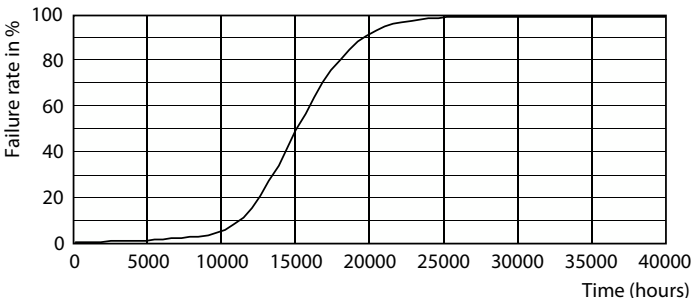
Life Expectancy Diagram - Ess LEDBulb 8-W E27 6500K A19 1PF/2 CO
