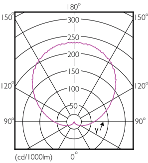
Light Distribution Diagram - Ess LEDBulb 8-W E27 6500K A19 1PF/2 CO
